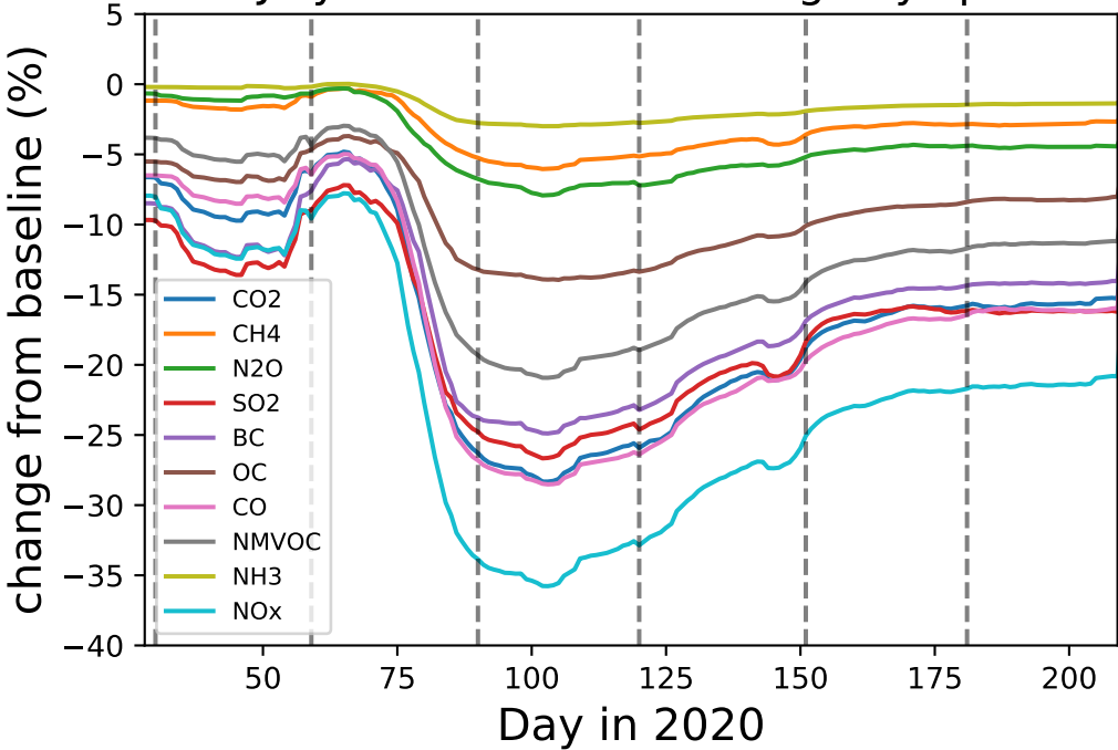
Feb-July 2020 emission change by species
